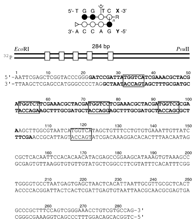
Figure 6. Sequence of the EcoRI / PvuII restriction fragment of the plasmid pAH2. The binding sites of interest are marked with boxes. The insert used in the cloning process is shown in bold face.
