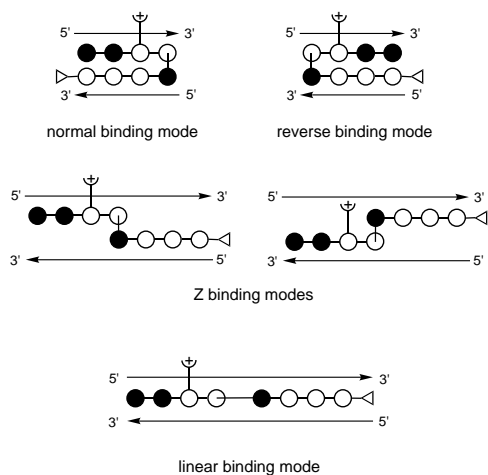
Figure 4. Representations of theoretically possible binding modes of U-pins. In the “normal” binding mode the N→C direction of the polyamide is parallel to the 5'→3' direction of the DNA, whereas in the reverse binding mode it is antiparallel. These two binding modes have been observed for hairpin polyamides with the latter occurring in some exceptional cases only. [10] Depending on the length of the bridge in the U-turn, binding in a previously unknown “Z binding mode” or—in case of longer bridges—in a linear (or 1:1) binding mode could also be theoretically possible. Since the upper and lower strands of the DNA are arbitrarily defined, the polyamide could of course also fit into the minor groove after a 180° rotation around an axis perpendicular to the helix axis—given an appropriate recognition pattern in the minor groove.
