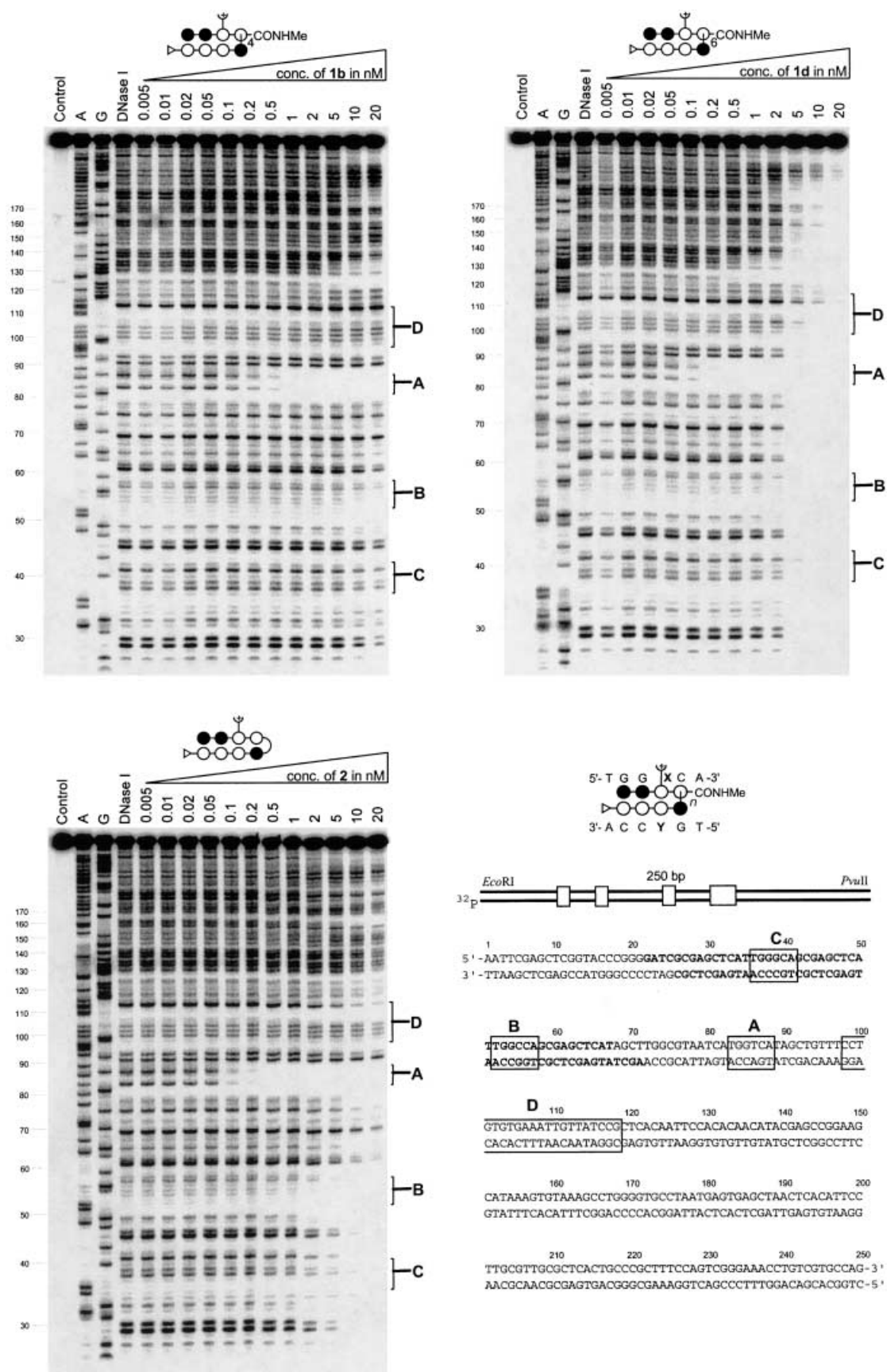
Figure 5. Results of DNase I footprinting experiments with the EcoRI/PvuII restriction fragment of the plasmid pDEH9 and the polyamides 1b , d and 2 . In the lower right corner the sequence of the restriction fragment is shown (insert used for cloning in bold-face) and the four binding sites of interest are labeled A, B, C and D (for a discussion see text). The only match site for such a U-pin is site A. The numbers indicate the position on the DNA fragment.
